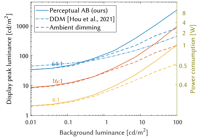
Fig. 9. Display auto-brightness curves. Continuous lines (Perceptual AB (ours)) show the lines of matching perceived contrast with respect to a reference display with contrast from 64:1 to 4:1 , which is observed with no ambient light. The dotted line presents another form of auto-brightness curve investigated with ergonomic study in a driving simulator [Hou et al., 2021]. The dashed lines show the same auto-brightness curves when ambient light dimming is used and the dotted lines follow the physical contrast. The right-hand y-axis shows the expected power consumption of Quest Pro, based on the data from [Chen et al., 2024].
