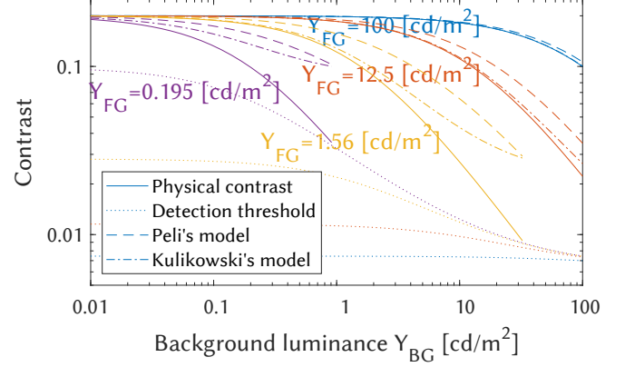
Fig. 6. The effect of ambient luminance on contrast in AR. The continuous lines show how the physical contrast is reduced (from c_{base} of 0.2) when the background light is added. The dashed and dot-dashed lines represent matched contrast according to two different models. The dotted lines show the detection thresholds used in the models (for 4 cpd patterns).
