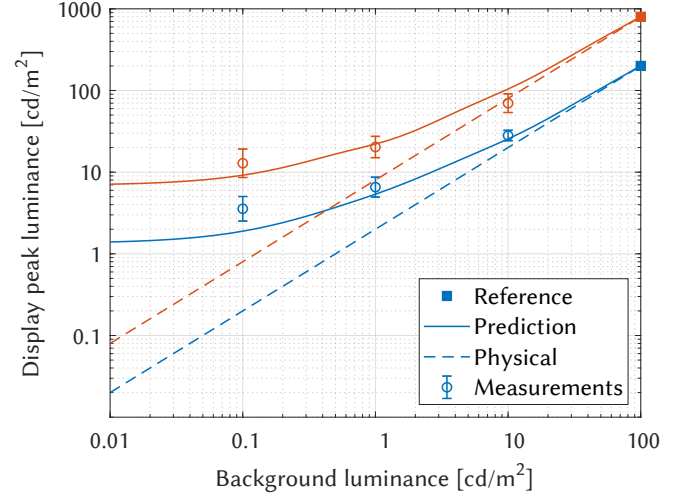
Fig. 8. Matching contrast of complex images in AR. The continuous lines represent the lines of matching contrast for a display that is affected by ambient light (x-axis) and has its peak luminance adjusted (y-axis). The circles with error bars (95% confidence intervals) show the results of Experiment 3. The two colors correspond to the two reference conditions (square) we used in Experiment 3 ( Y_{\text{dmax}}^{\text{ref}} = 200 and Y_{\text{dmax}}^{\text{ref}} = 800 \text{ cd/m}^2 ). The dashed lines represent matching physical contrast. Per-image results can be found in the supplementary Fig. S8.
